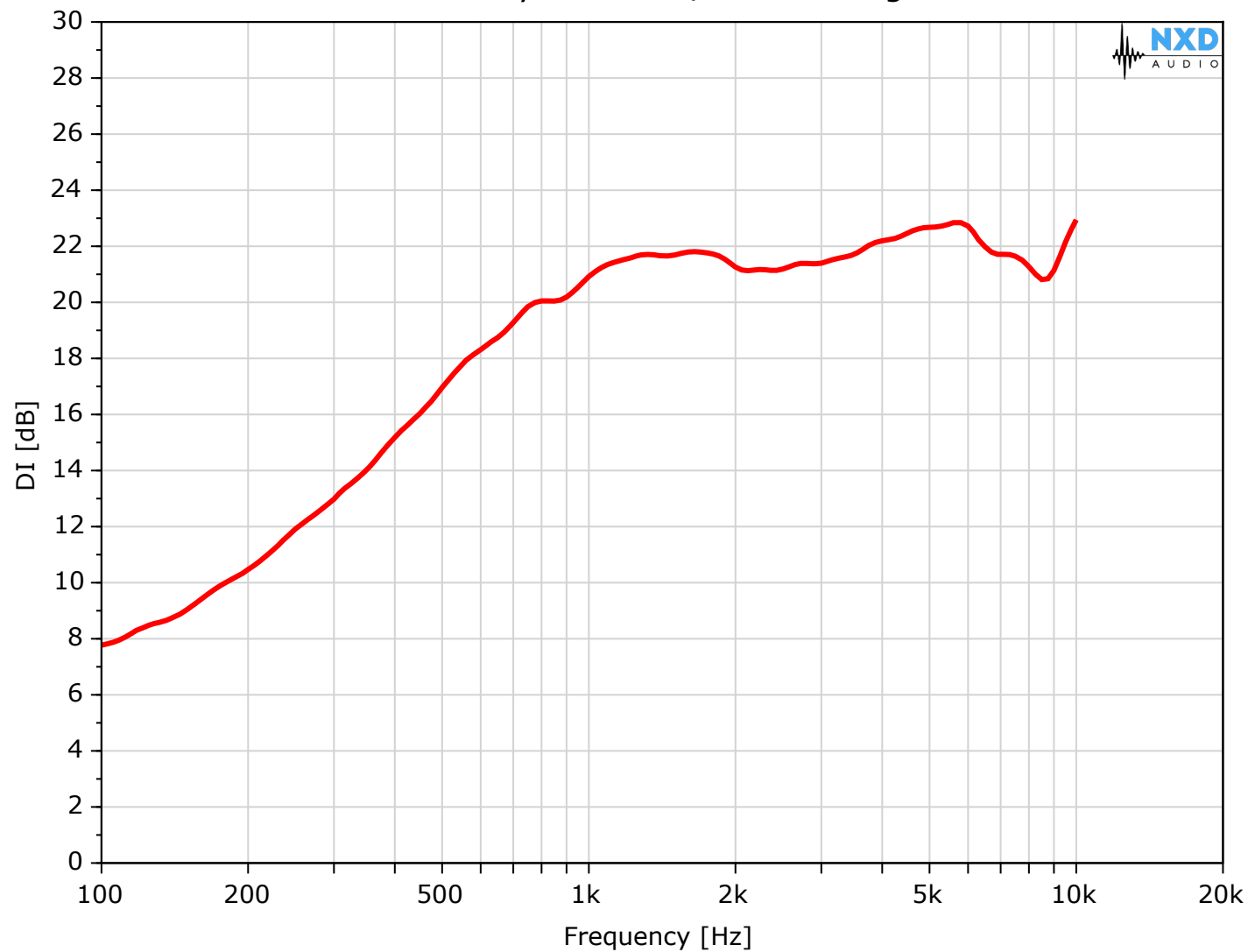
Directivity Index - 1/3 oct averaged
