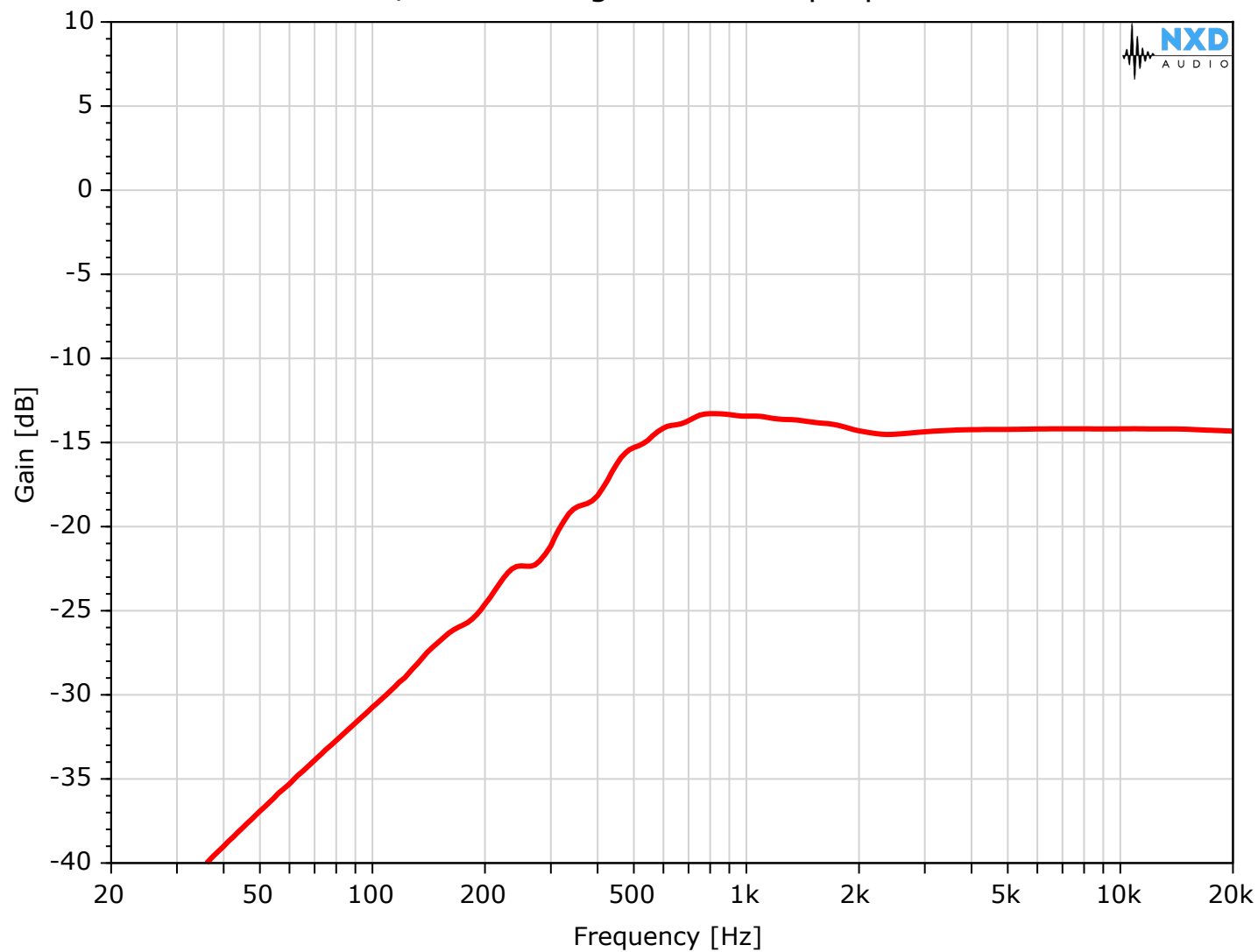
Filter - 1/3 oct averaged - 50 W tap - protection on
