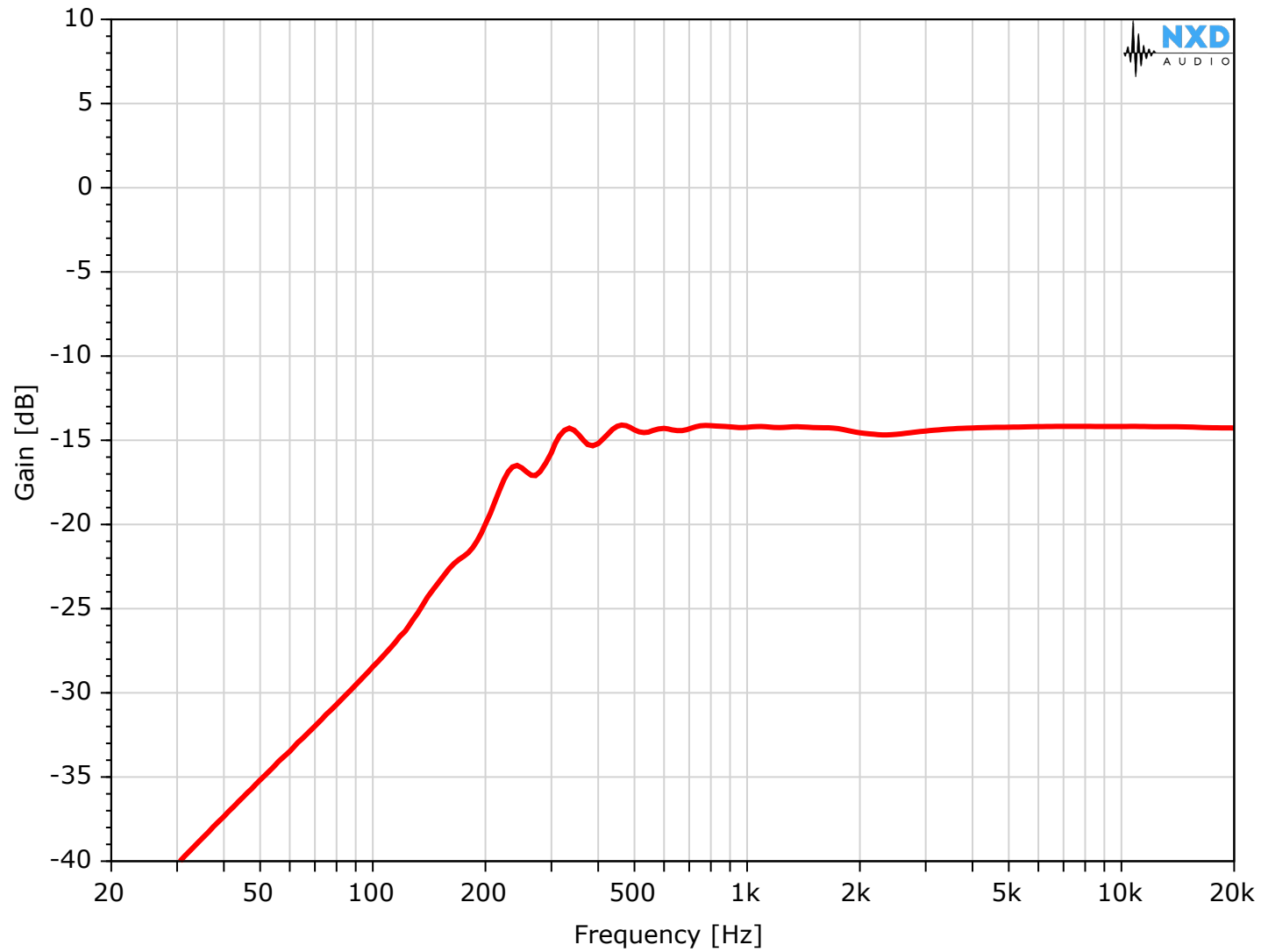
Filter - 1/3 oct averaged - 50 W tap
