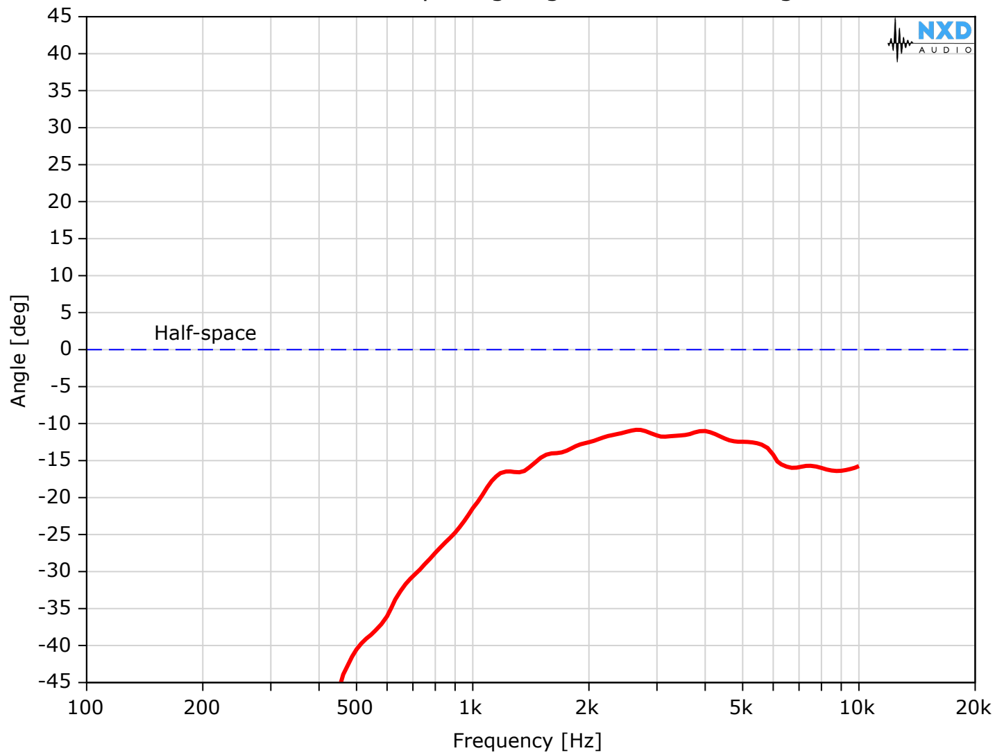
Vertical -6 dB opening angle - 1/3 oct averaged
