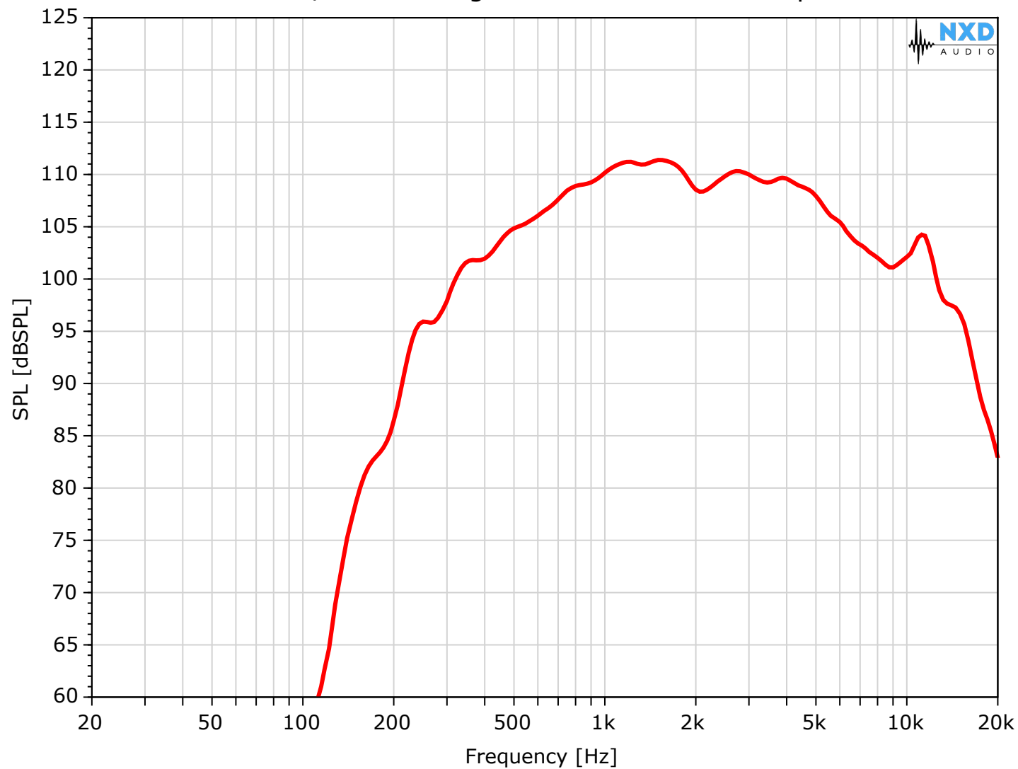
SPL - 1/3 oct averaged - 10 V at 4 m - half-space
