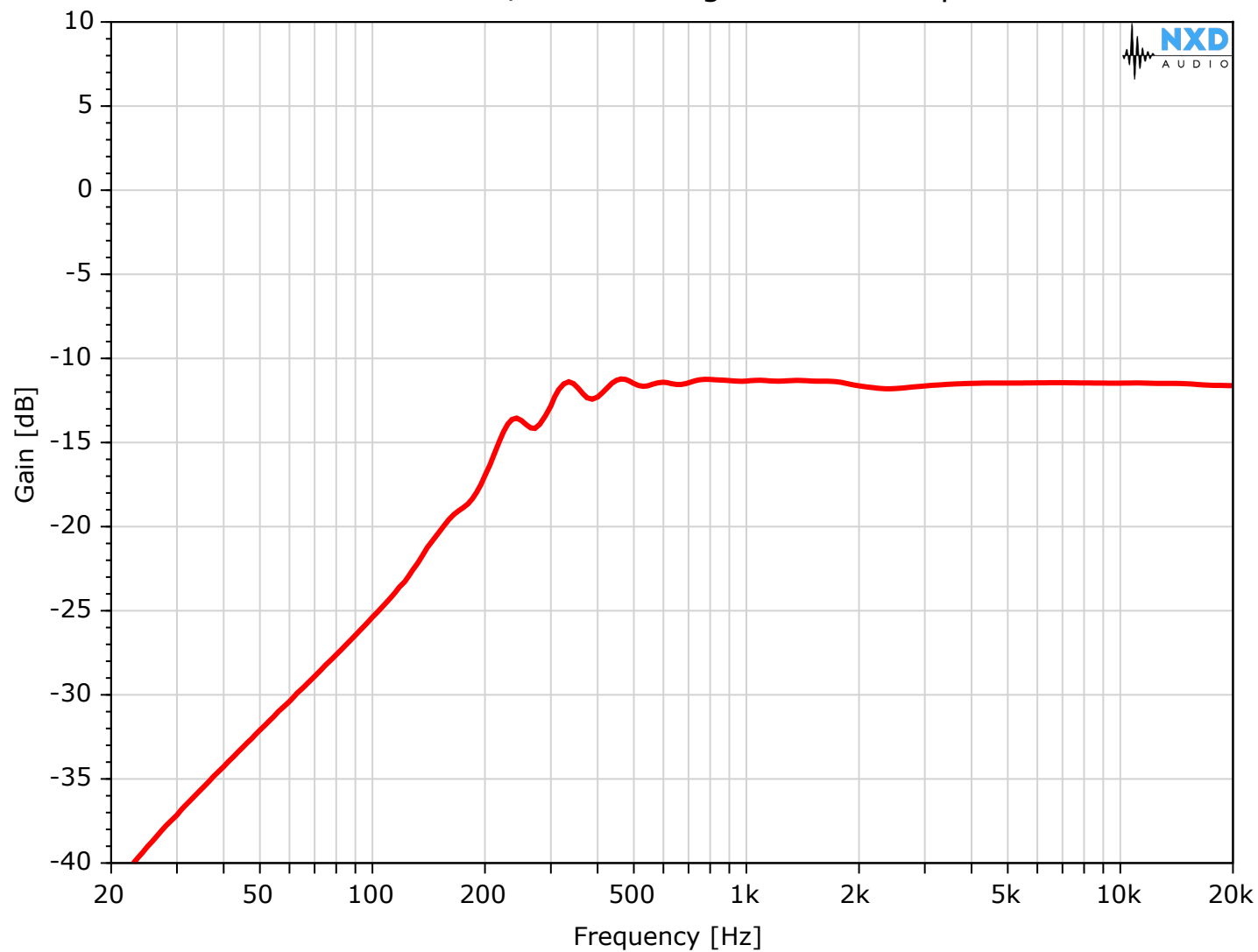
Filter - 1/3 oct averaged - 100 W tap
