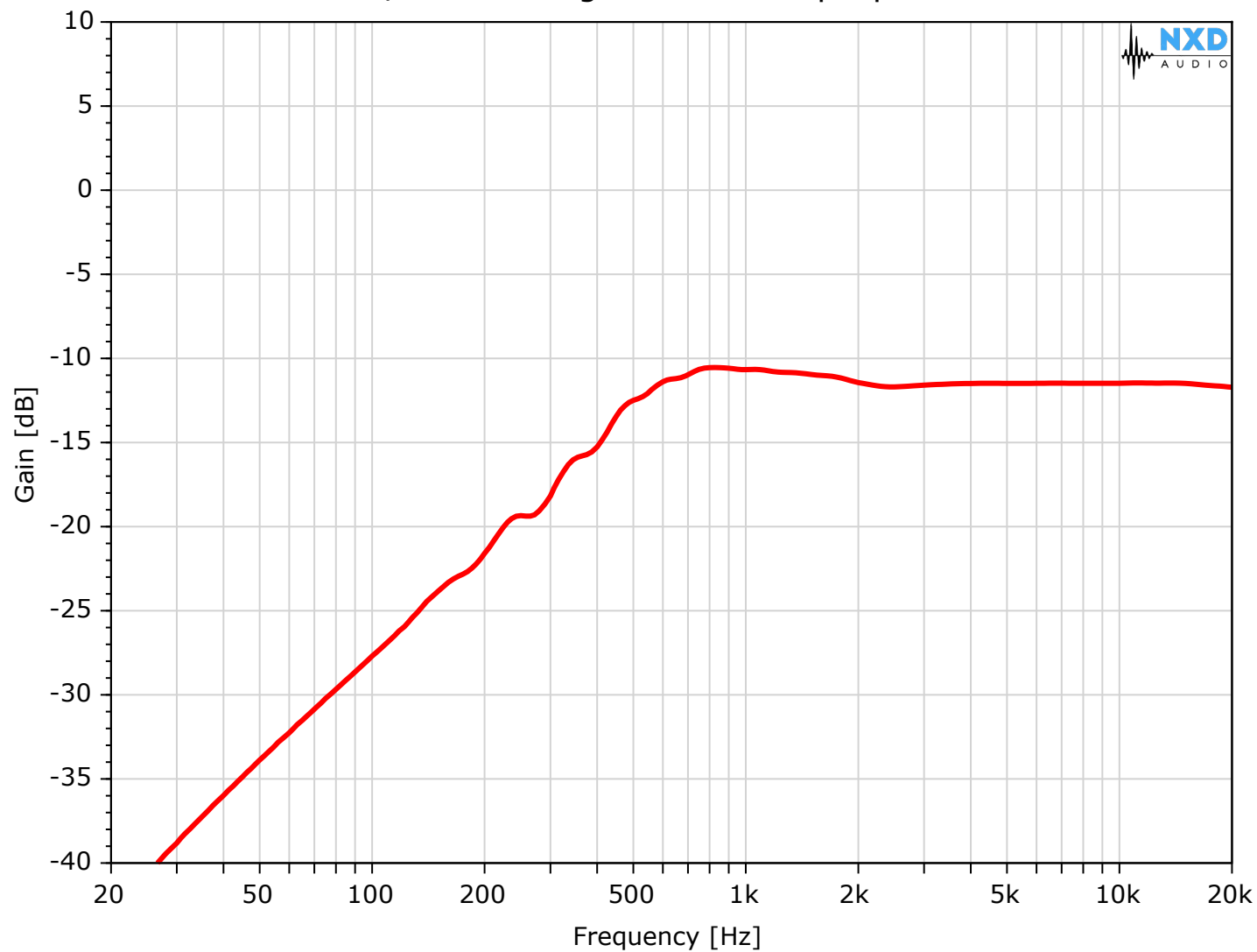
Filter - 1/3 oct averaged - 100 W tap - protection on
