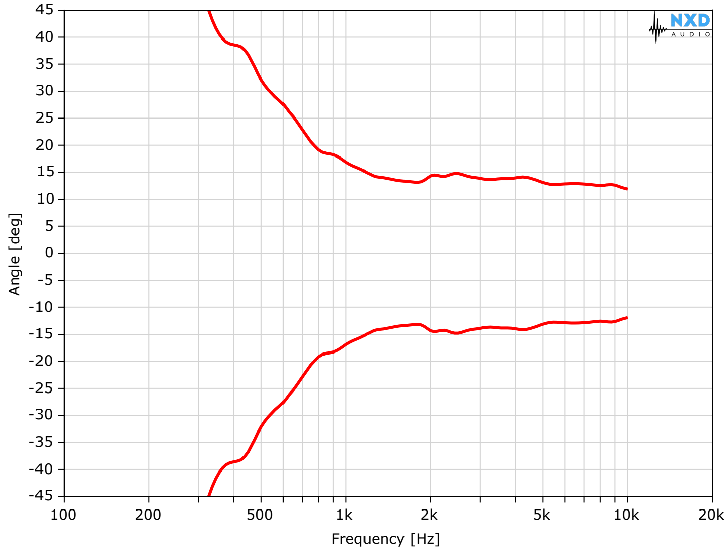
Horizontal -6 dB opening angle - 1/3 oct averaged
